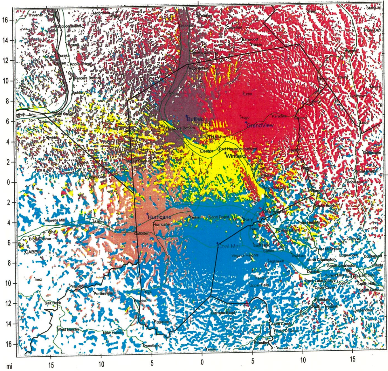
Putnam Existing VHF Portable Talk Back Most Likely Server
