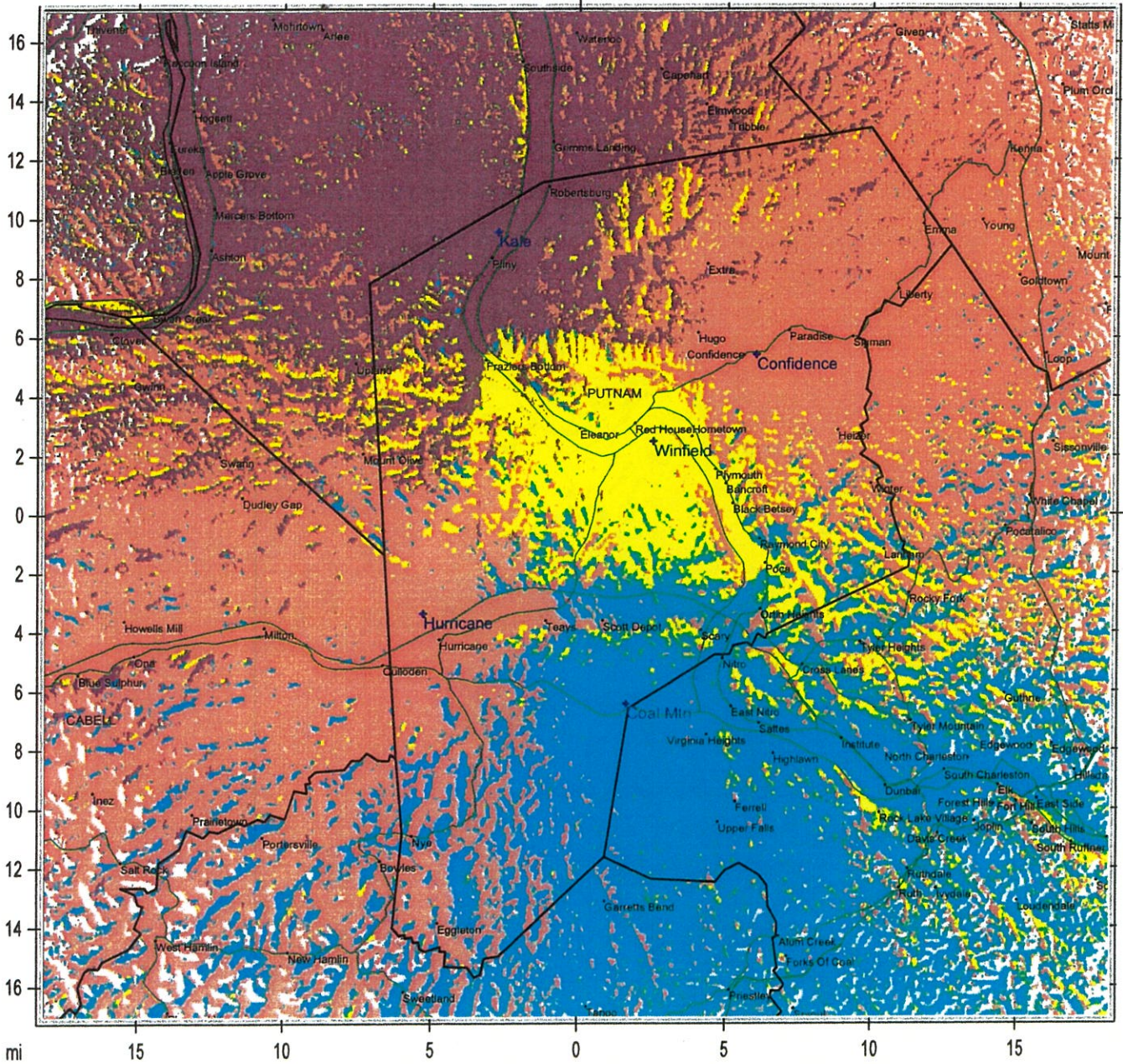
Putnam Proposed VHF Mobile Talk Back - Most Likely Server
