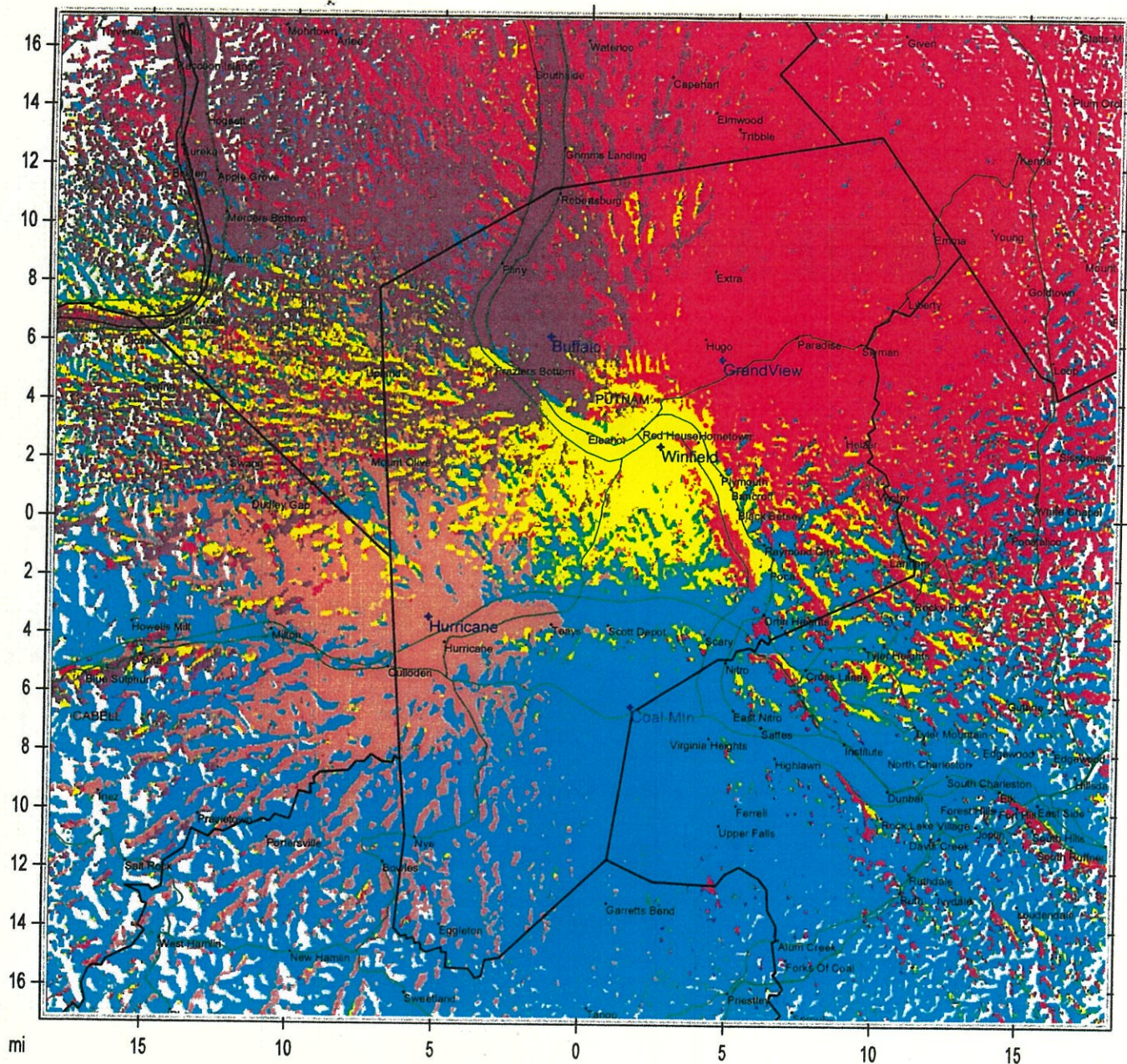
Putnam Existing VHF Talk Back Most Likely Server (MLS)
